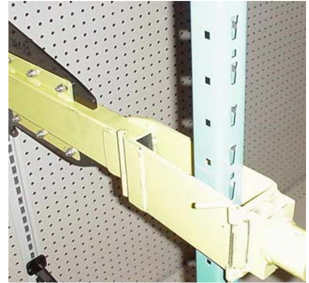
SPECIAL ARM -TO LIFT OUTRIGGER
